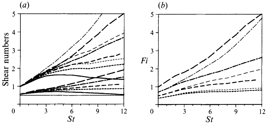
FIGURE 9. (a) Shear number Sh = Sl/q (upper curves) and SGS shear-number Sh_{sgs} = S\Delta x/(2e)^{0.5} (lower curves) versus St , (b) inverse Froude number Fi = Nl/q versus St . Line coding as in figure 2.
