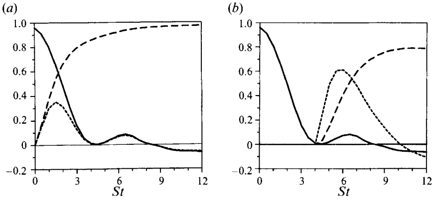
FIGURE 21. Correlation coefficients versus St (DNS data); (a) for release of c_3 at St = 0 , (b) for release of c_3 at St = 4 ; —, -\overline{w\theta}/(w'\theta') ; ---, -\overline{wc_3}/(w'c'_3) ; —·—, \overline{\theta c_3}/(\theta'c'_3) .
