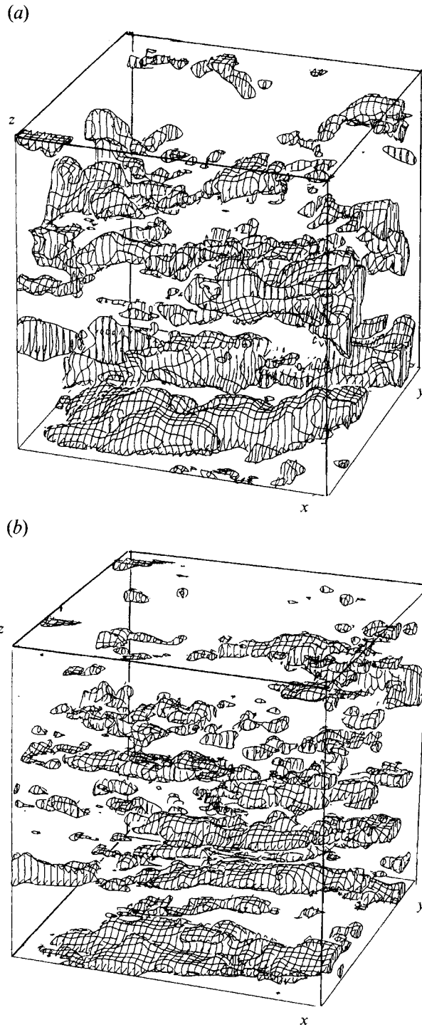
FIGURE 11. Perspective views of iso-surfaces of concentration fluctuation c_1 \approx 1.3c'_1 in a subdomain with side-lengths \frac{1}{2}L at St = 12 for (a) Ri = 0 , (b) Ri = 0.5 . These results are from simulations with 96^3 grid points.
