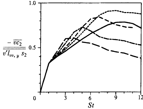
FIGURE 23. Test of mixing-length model, equation (20), for a flux driven by a cross-stream gradient. Line coding as in figure 2.
