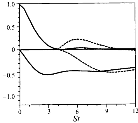
FIGURE 22. Normalized diffusivity tensor components D_{33}/D_{22} (upper curves) and D_{13}/D_{22} (lower curves) versus St computed by heat fluxes: —, computed by scalar fluxes (release at St = 4 ): ----. The curves computed by the fluxes of the scalar released at St = 0 have been omitted since they are indistinguishable from the solid lines already for St > 0.5 .
