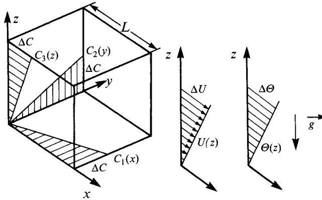
FIGURE 1. Computational domain and mean profiles.
