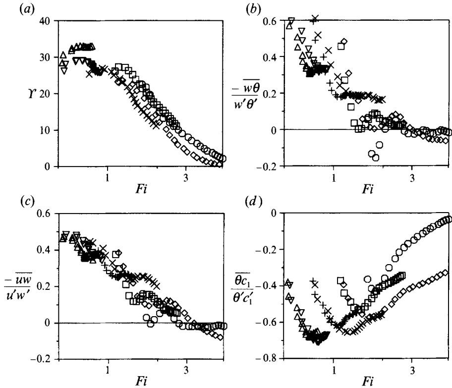
FIGURE 10. Percentage of convective instabilities Y (a), correlation coefficients of vertical fluxes of heat (b), downstream momentum (c), and correlation coefficient \overline{\theta c_1}/(\overline{\theta' c_1'}) (d) versus inverse Froude number Fi at St \geq 2 . Symbols for LES: \triangle , Ri = 0.13 ; + , 0.25 ; \square , 0.5 ; \circ , and 1 ; symbols for DNS; \nabla , Ri = 0.13 ; \times , 0.25 ; \diamond , 0.5 . All data for Pr_{sgs} = 1 .
