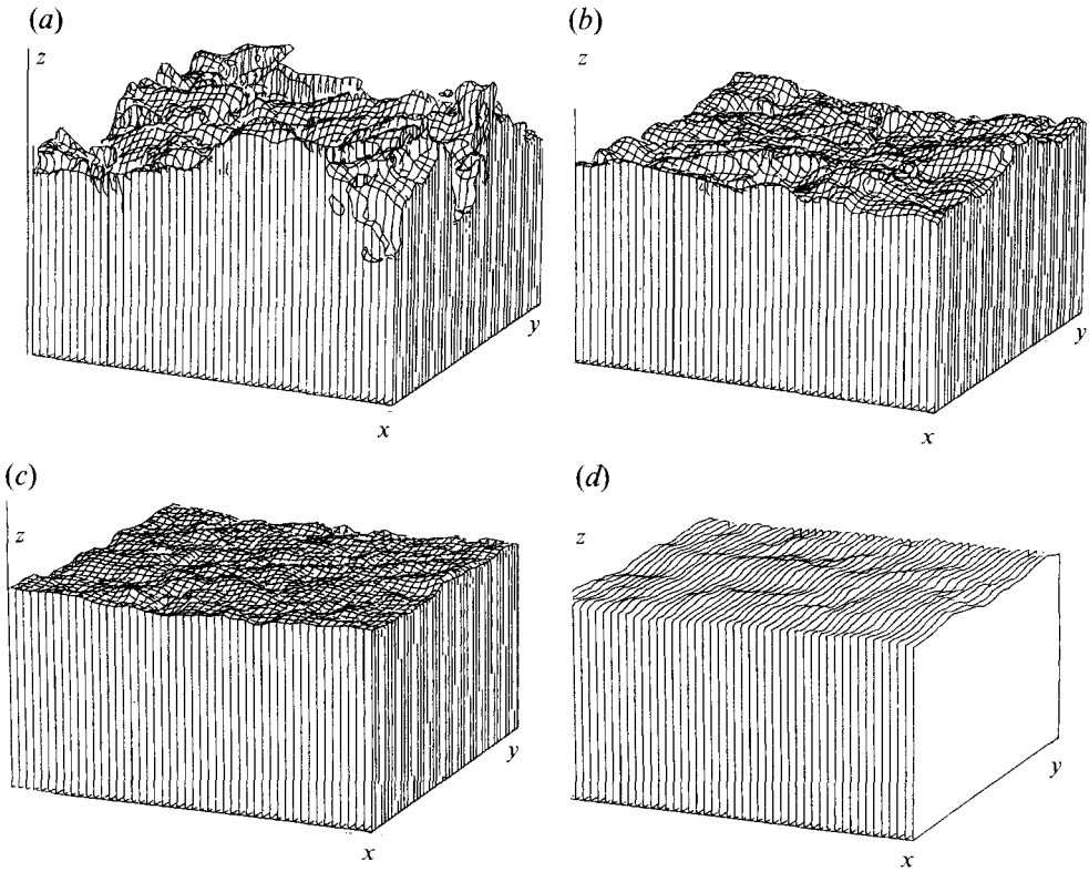
FIGURE 8. Perspective views of iso-surfaces of temperature \theta + \Theta = 0.25\Delta\Theta in a subdomain with side-lengths \frac{1}{3}L at St = 12 for various Richardson numbers. These results are from simulations with 96 3 grid points. (a) Ri = 0 , (b) Ri = 0.25 , (c) Ri = 0.5 , (d) Ri = 1 .
