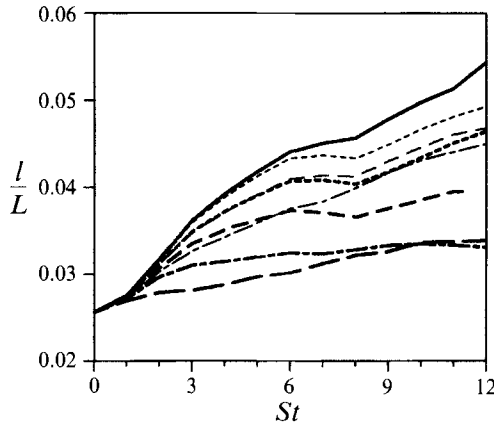
FIGURE 7. Integral lengthscale l/L versus St with line coding as in figure 2.
